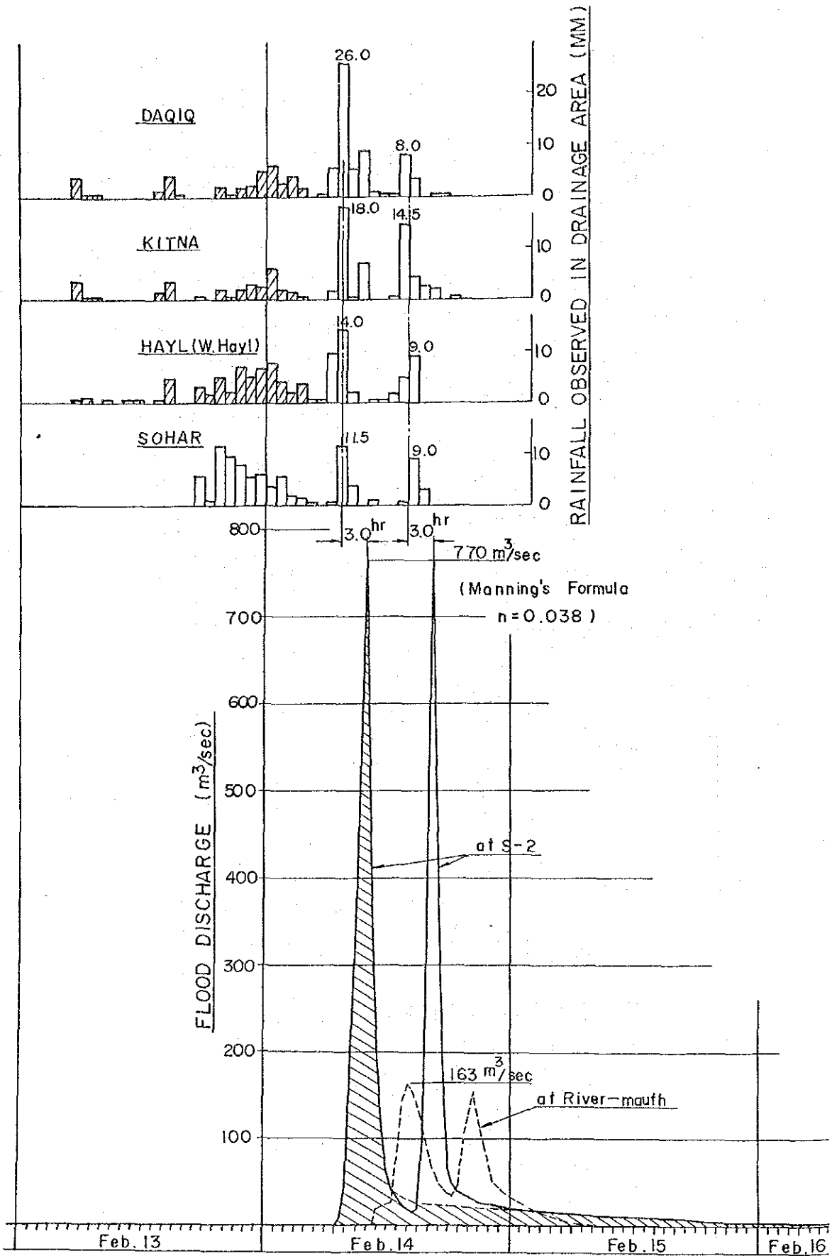
Figure A-3-5 Observed Flood in February 1982
