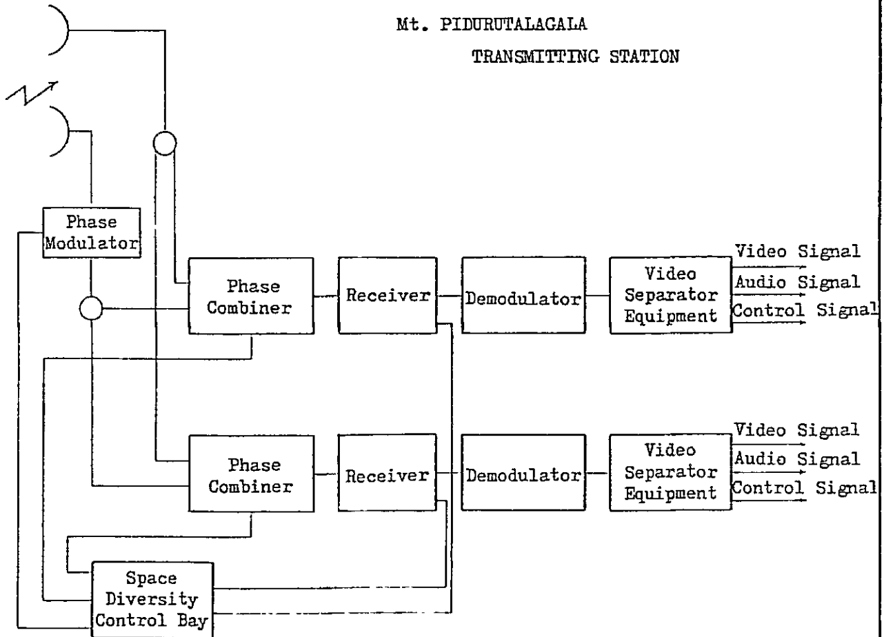
Fig1-1 SCHEMATIC DIAGRAM OF MICROWAVE LINK ( FROM COLOMBO TO Mt. PIDURUTALAGALA )
