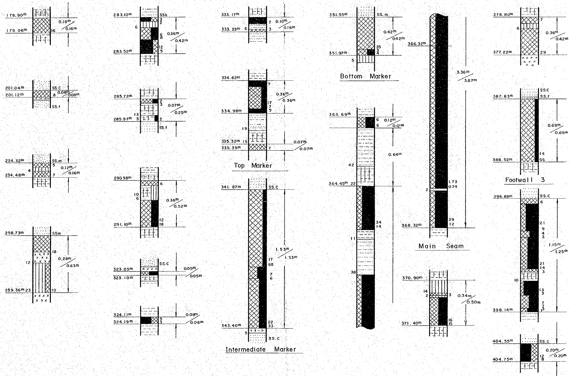
DRAWING 8b. COAL SEAM COLUMNAR SECTION OF DD25 Scale = 1:20
