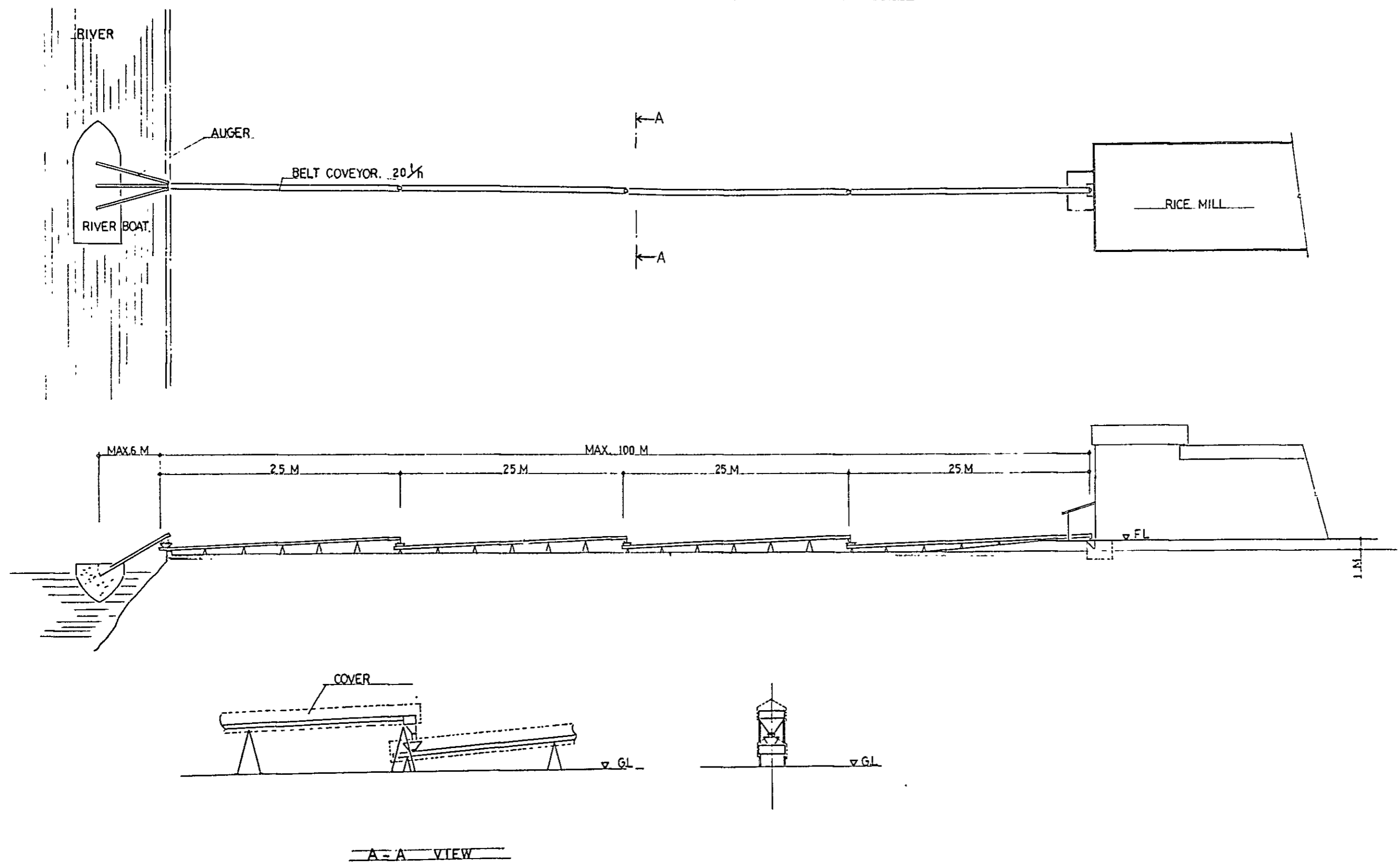
Fig. 26 UNLOADING & TRANSPORTATION FACILITY, BASSEIN, KANAUNGTOE, DEDAYE & EINME
