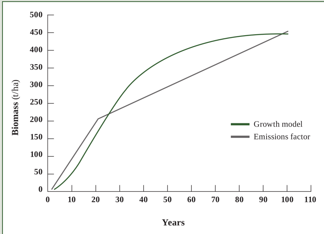
Figure 5: Comparison of an emissions/removals factor model and a typical growth curve
