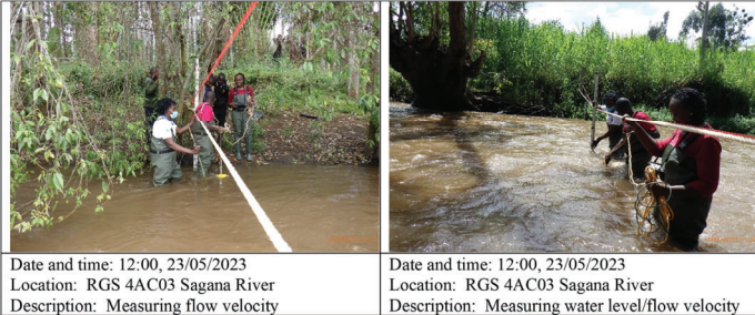
Discharge measurement at 4AC03 Sagana
