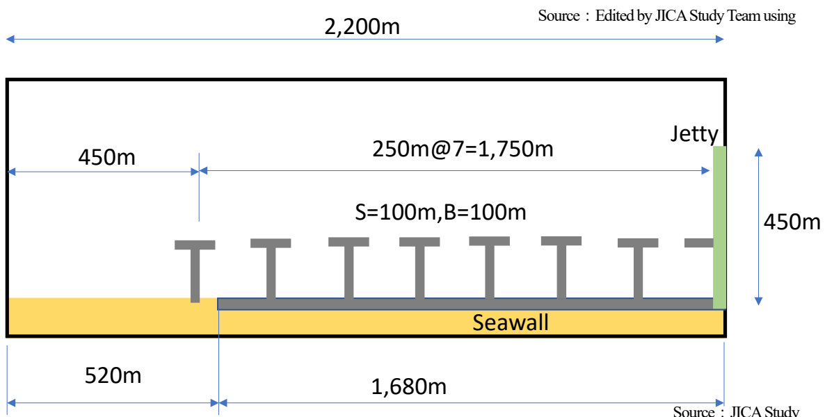
Figure 50 Modeled Topography and Coastal Facility Plan (Pemalang-Pekalongan S-4a)
