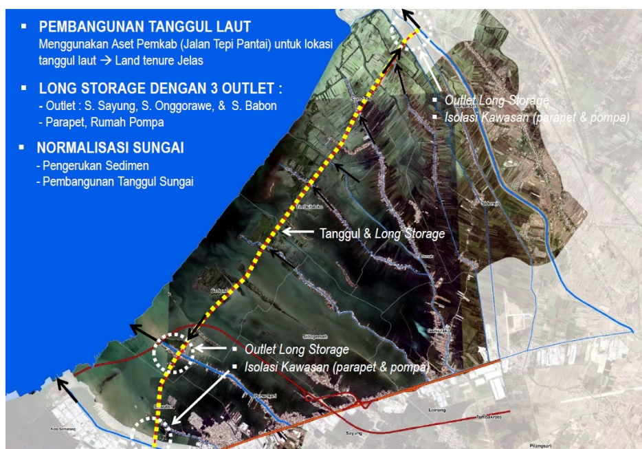
Figure 28 Diagram of Seawall Layout
