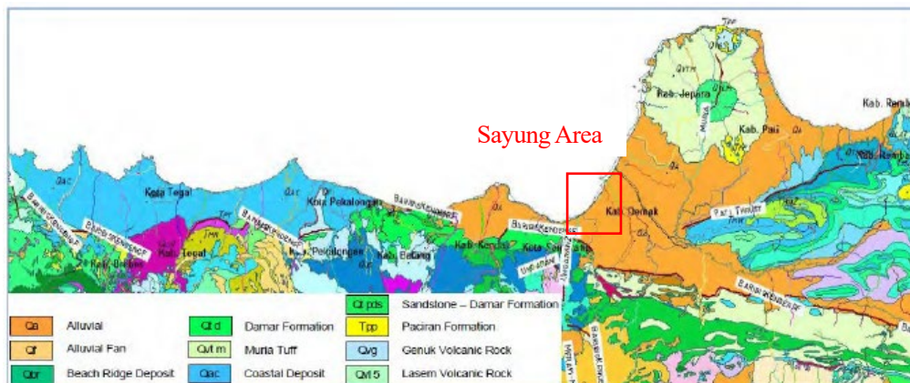
Figure 3 Geological Map of Central Java
