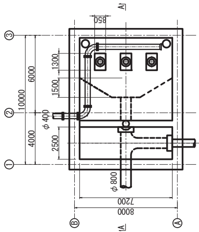
First basement floor plan
