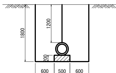
Typical Section for Open-cut Method S=1/70
