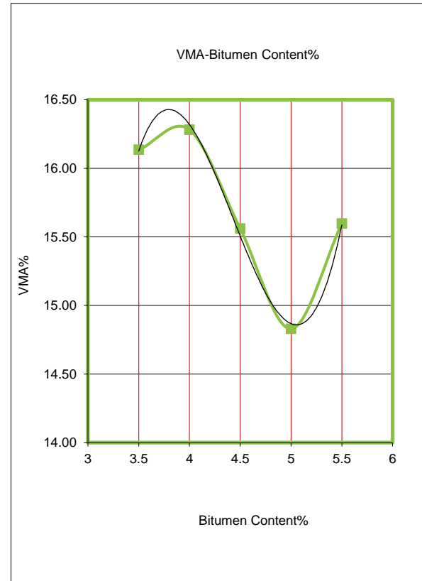
Bitumen content vs VMA
