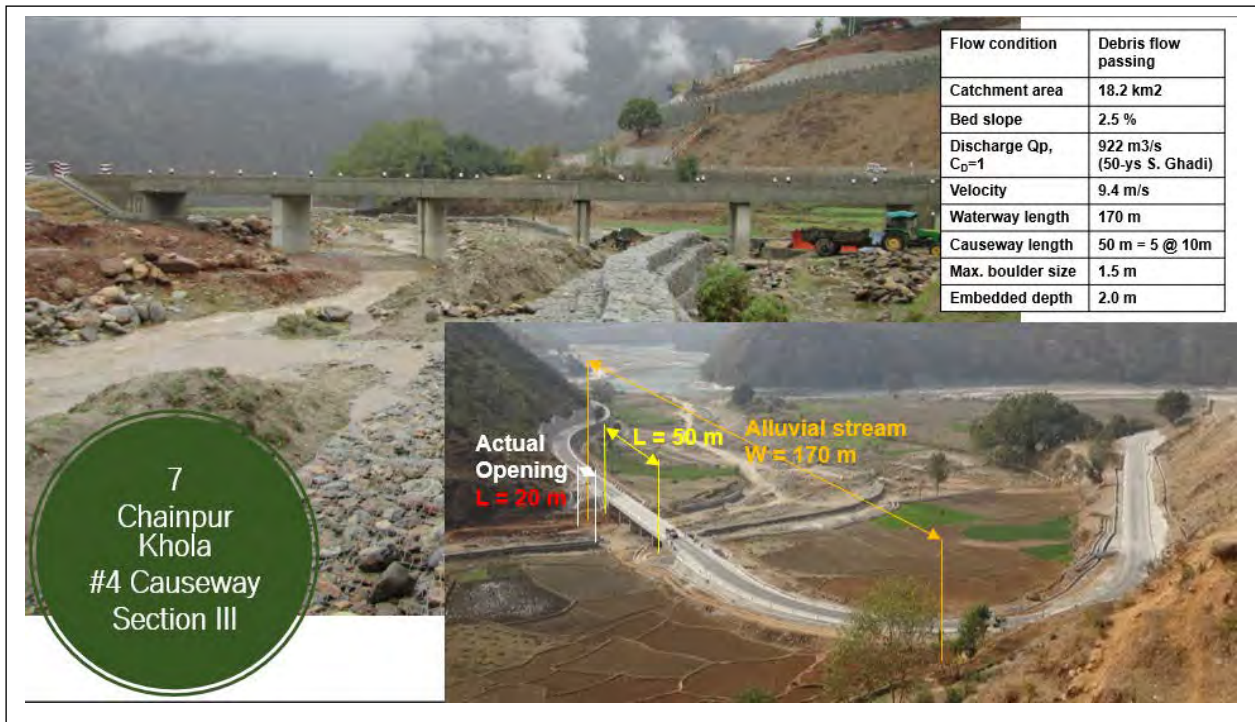
Figure 5-3 Present Condition of Chainpur Khola Causeway, Sindhuli Road (Section-III)
