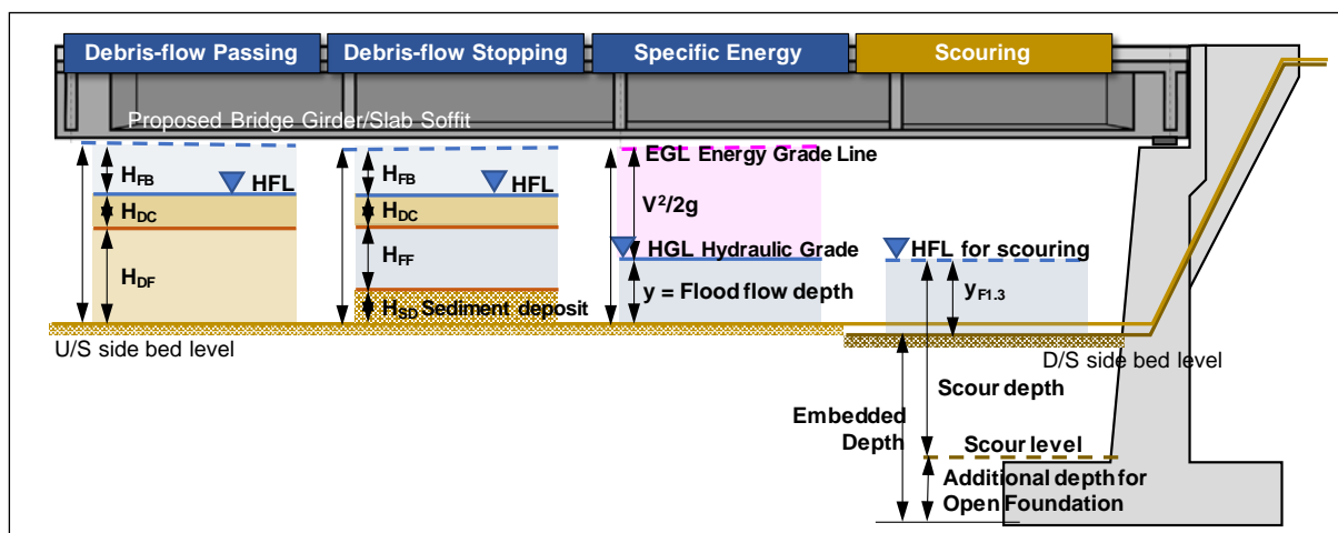
Figure 5-8 Definition Sketch of Vertical Clearance for Open Foundation
