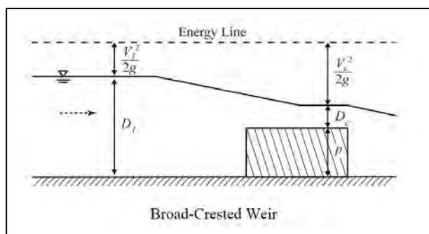
Figure 4-7 Definition Sketch of Broad Crested Weir
