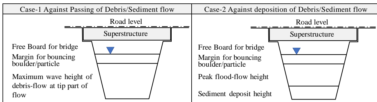
Figure 5-6 Definition of Two Cases of Vertical Clearance
