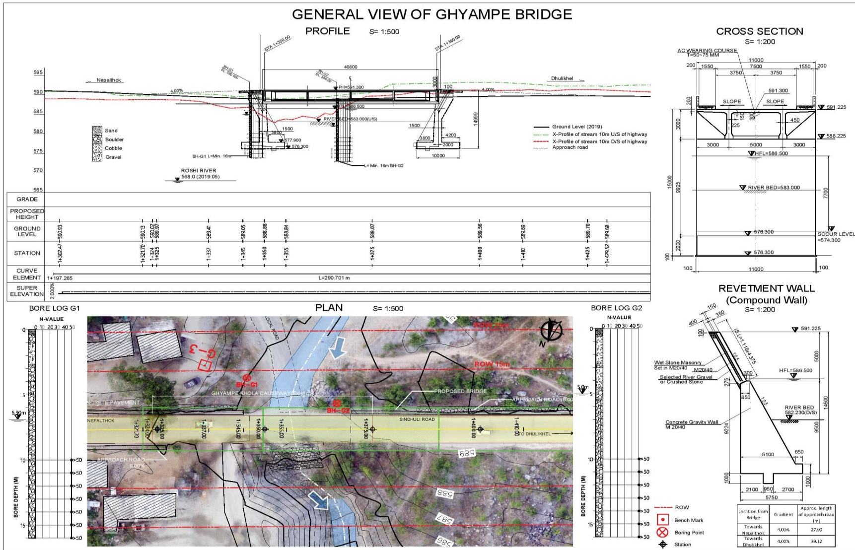
Figure 2- 2: General View of Ghyampe Bridge
