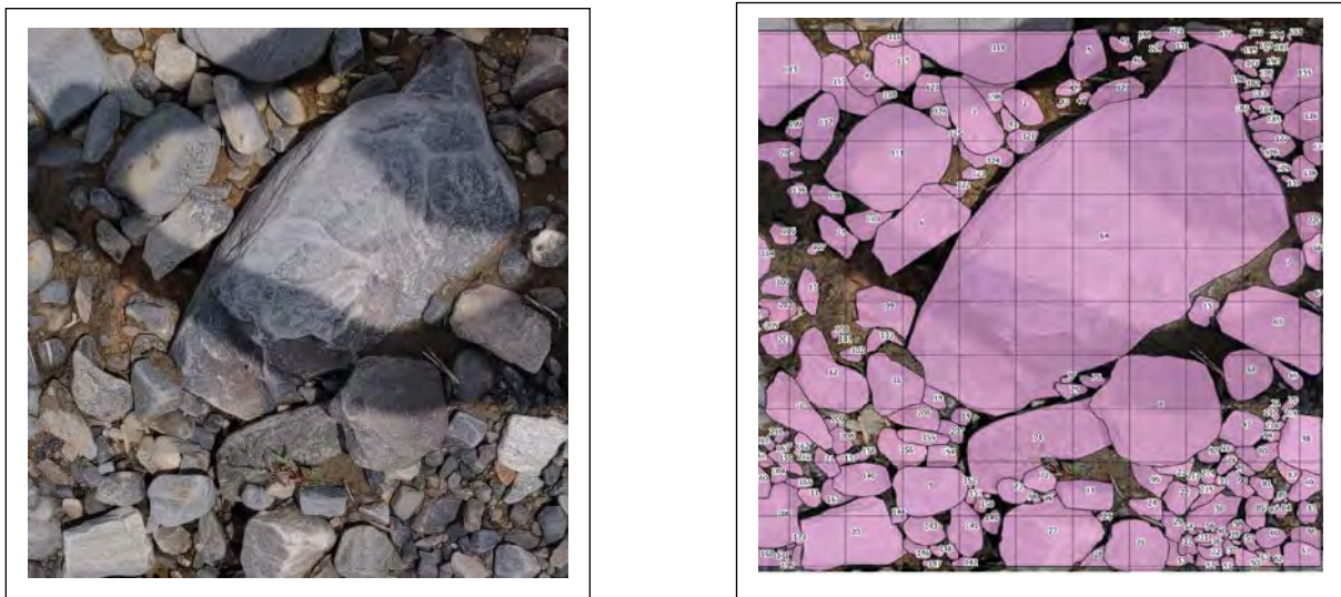
Figure 5-10 Image Analysis for Sieve Grading
