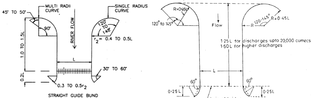
Fig. 8.16. Gale's recommendations for guide banks.
