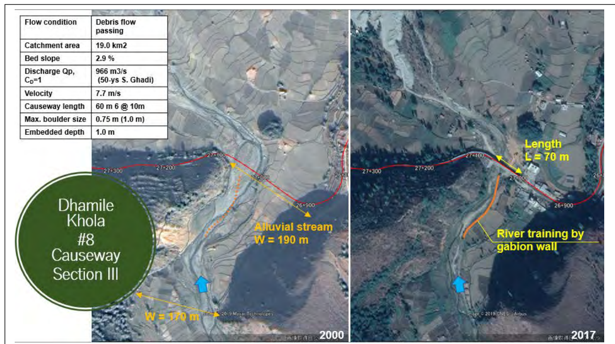
Figure 5-4 Present Condition of Gangate Khola Causeway, Sindhuli Road (Section-III)
