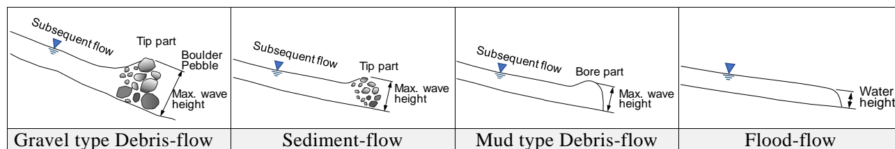
Figure 5-2 Pattern Diagram of Flow Type and Maximum Wave Height
