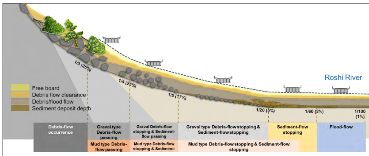
Figure 5-1 Riverbed Gradient and Nature of Debris-flow
