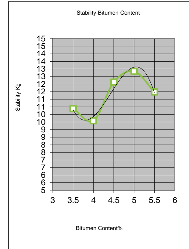
Bitumen content vs Stability
