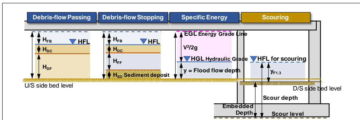
Figure 5-9 Definition Sketch of Vertical Clearance for Raft Foundation
