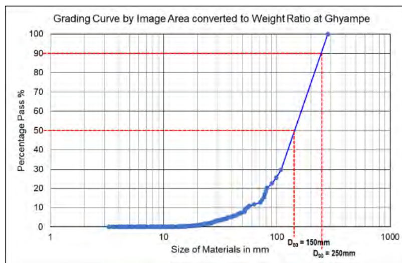
Figure 5-11 Representative Graph of Image analysis of Particle Size Distribution at Ghyampe
