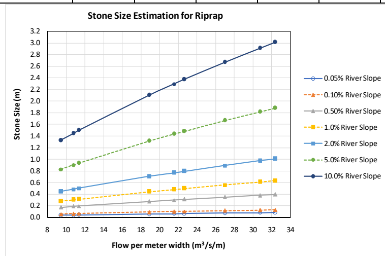
Figure 7-3 Size of Rip-rap Stones
