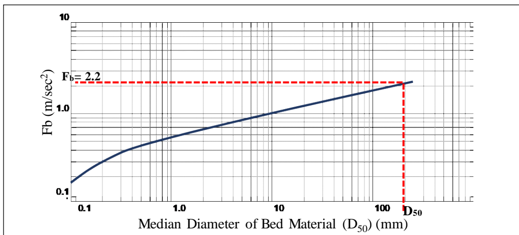
Figure 5-12 Blench F_b “Zero bed factor”
