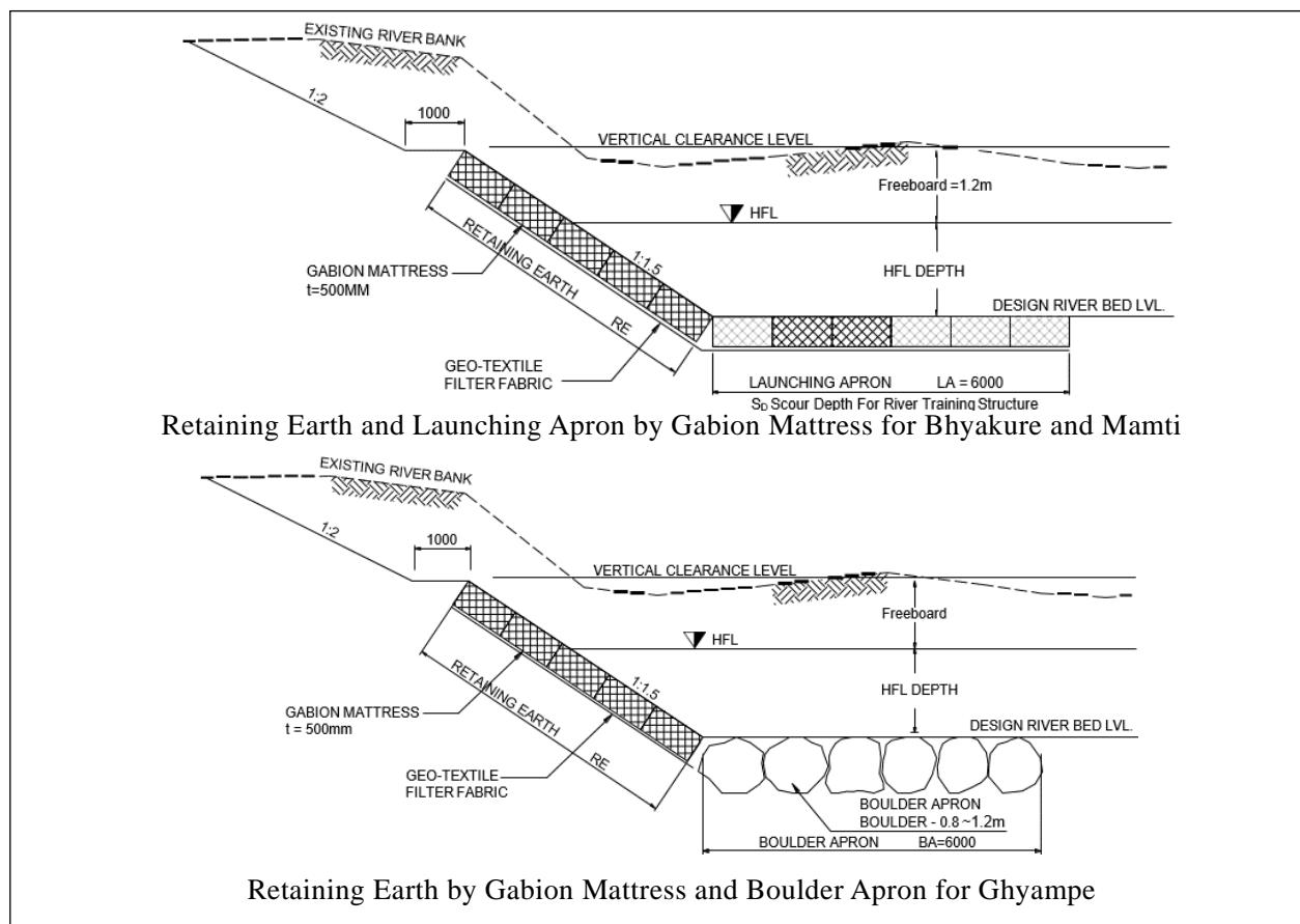
Figure 7-2 Designed Guide Bank
