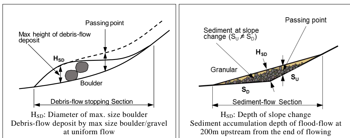
Figure 5-7 Definition Sketch of Debris-flow and Sediment-flow
