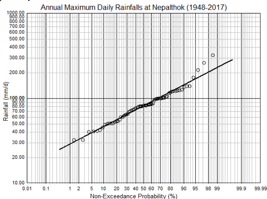
Figure 4-3 Lognormal Distribution Fitting of Maximum Rainfall of Nepalthok
