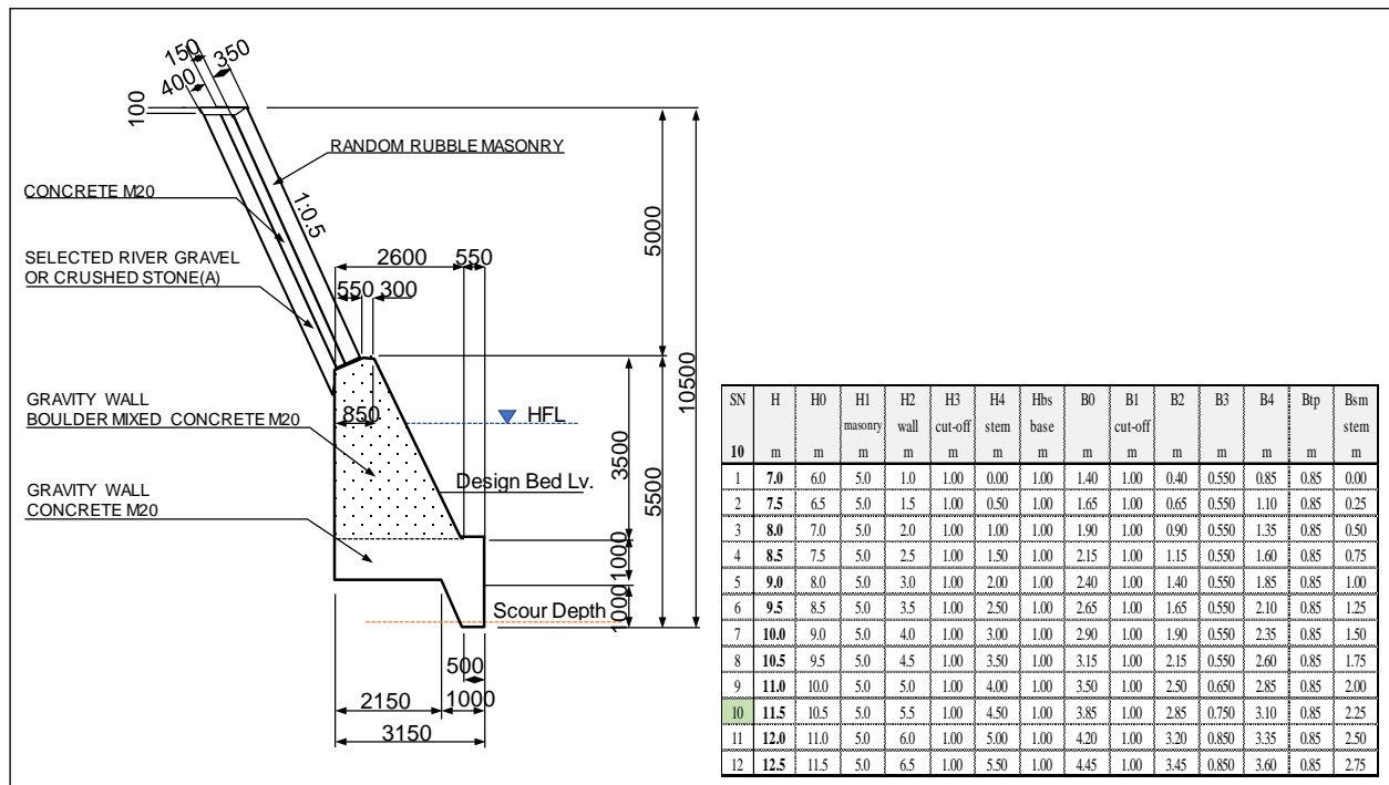
Figure 7-1 Designed Compound Wall
