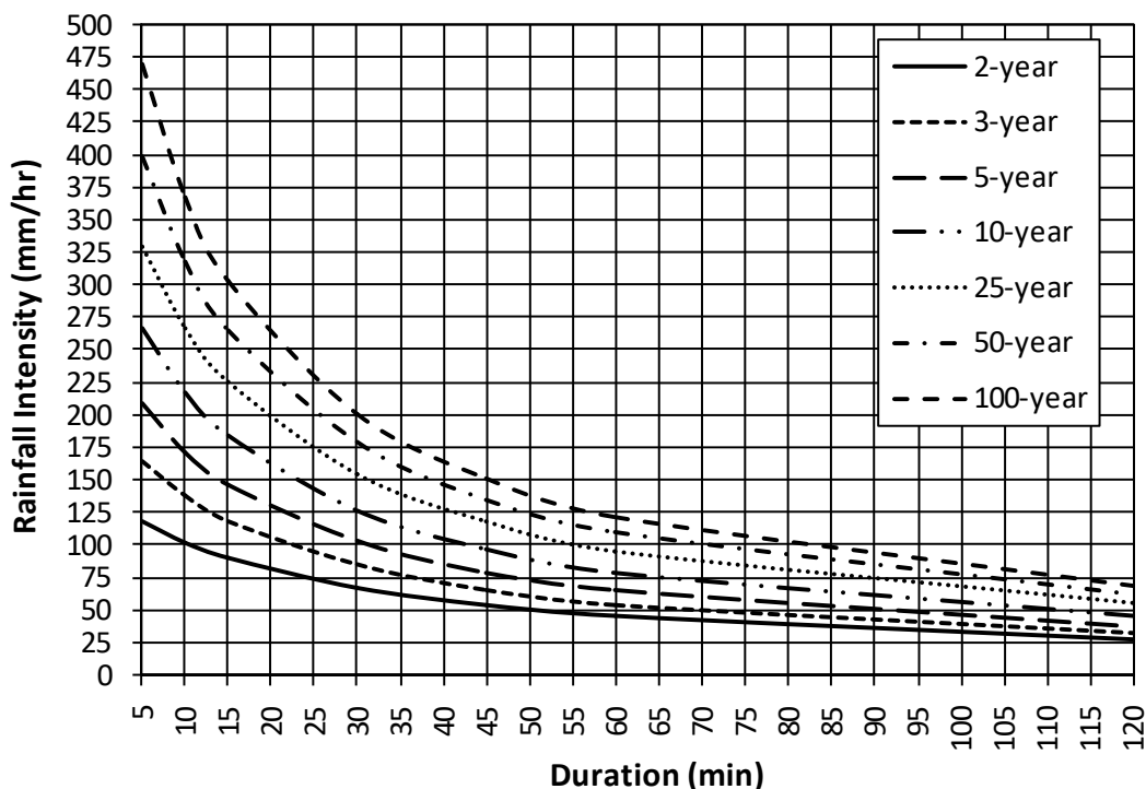
Figure 4-5 The IDF-Curve of Nepalthok
