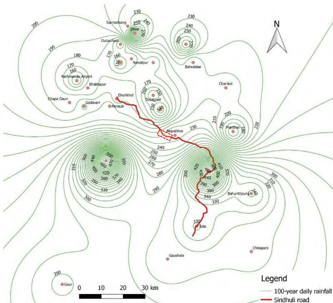
Figure 4-4 Isohyets of 100-year Daily Rainfall of the Project Area
