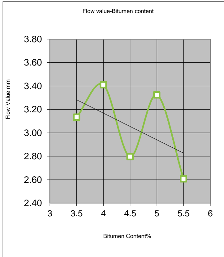
Bitumen content vs Flow Value
