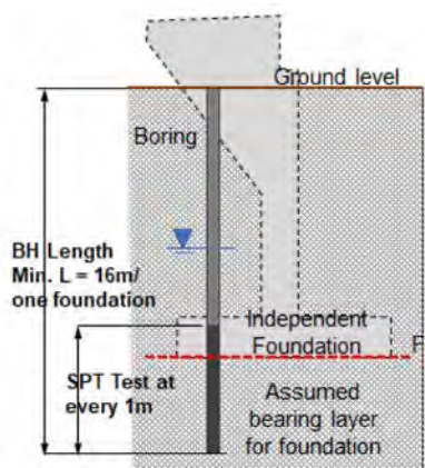
Figure 3-1 Arrangement SPT
